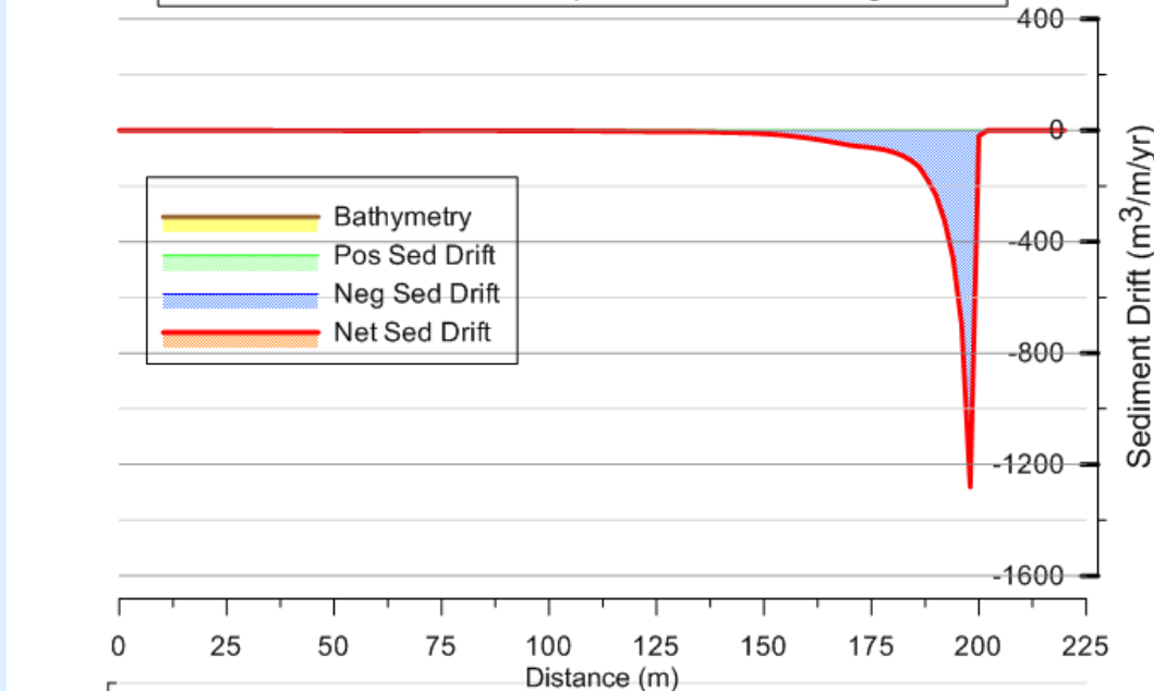
Cross-Shore Sediment Transport Distribution Along Profile1
