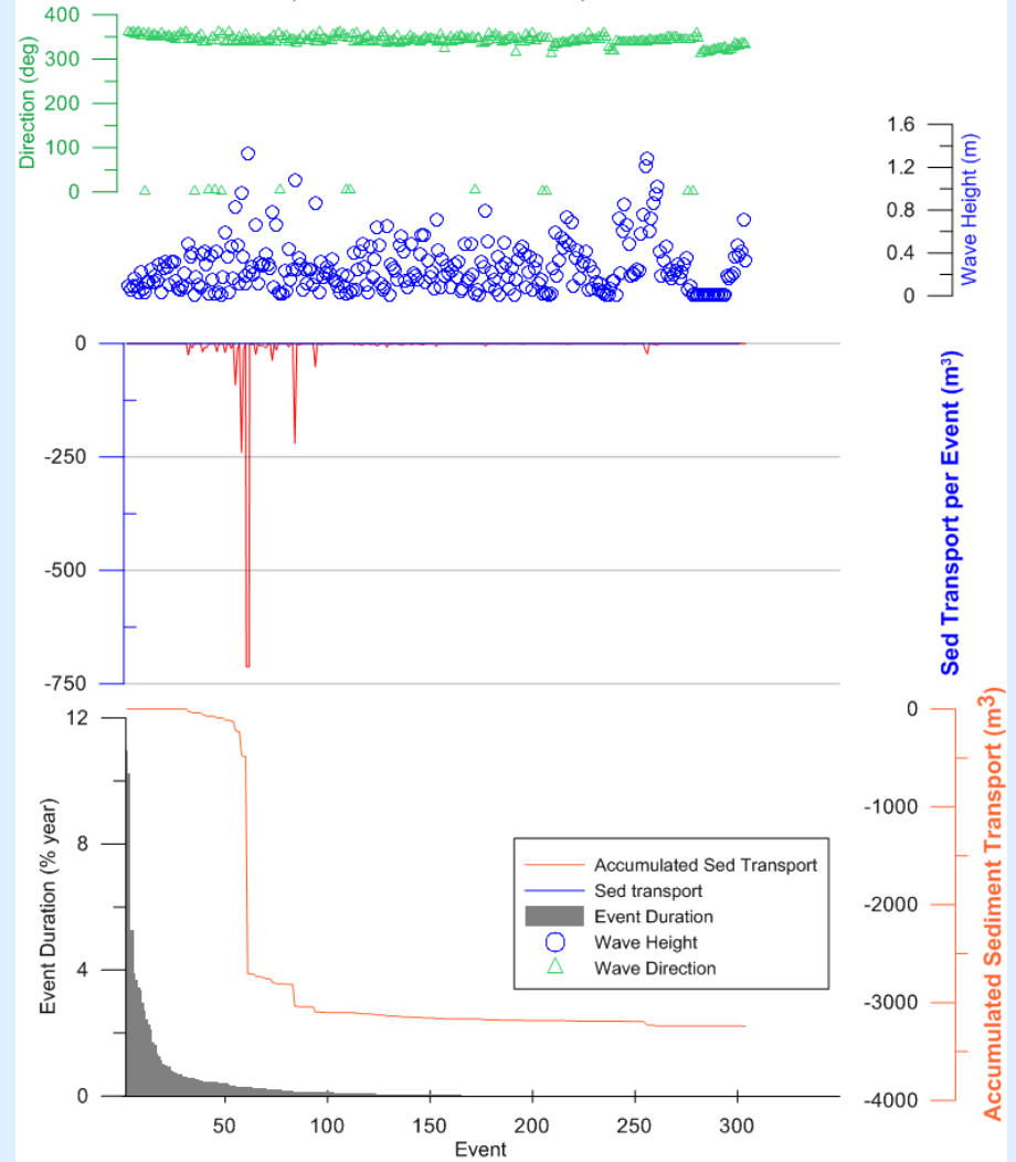
Sediment Transport at Profile 7 Cumulated per Wave Event and Duration
