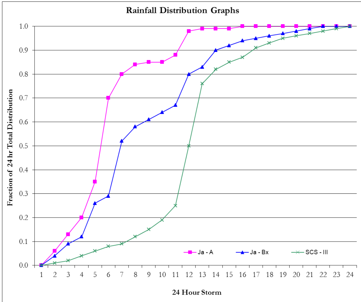
Figure 5.2 Rainfall distribution graphs applicable to Jamaica
