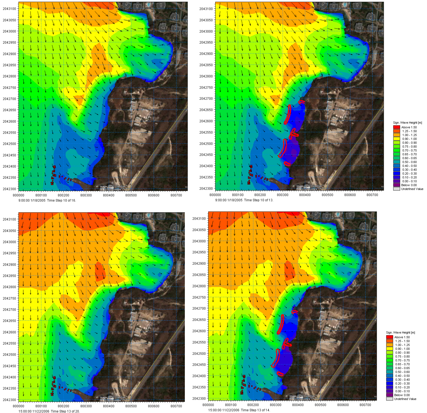
Figure 6.3 Significant wave height and direction at the peak of the winter 2005 swell event(top) and winter 2006 swell event(bottom) with existing (left), and proposed option (right)
