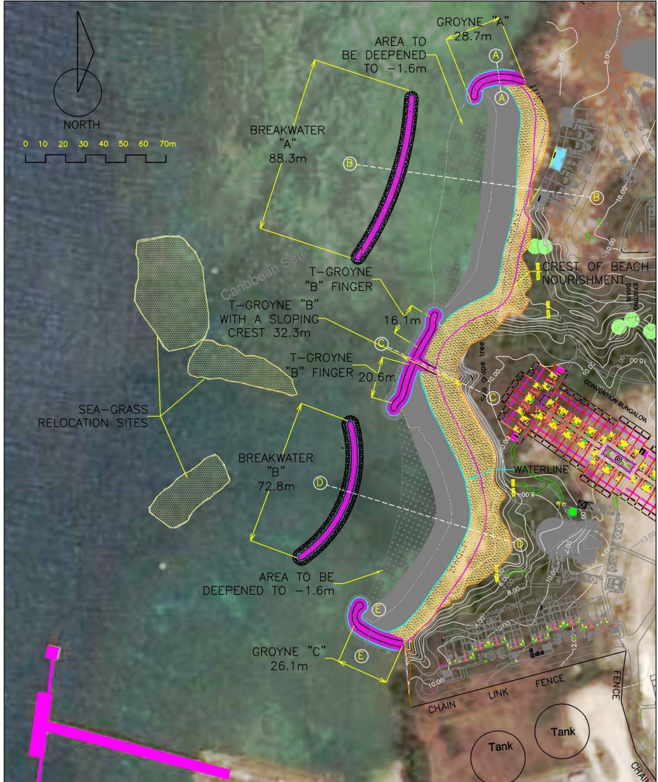
Figure 6.1 Proposed beach enhancement concept for the Grand Palladium Royal Suites with extended dry beach and swimming are as recommended by Fiesta Hotel Group
