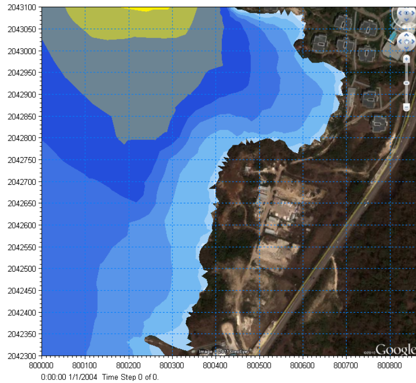
Figure 5 Maximum wave heights (Left) and storm surge (Right) for the 50 year hurricane event coming from east
