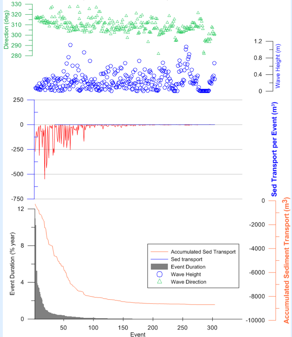
Sediment Transport at Profile 1 Cumulated per Wave Event and Duration
