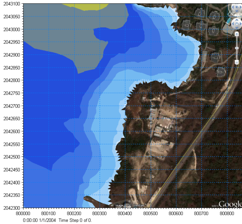
Figure 7 Maximum wave heights (Left) and storm surge (Right) for the 50 year hurricane event coming from west
