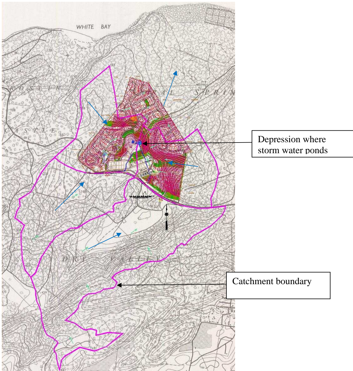
Figure 3: Catchment area for internal depression
