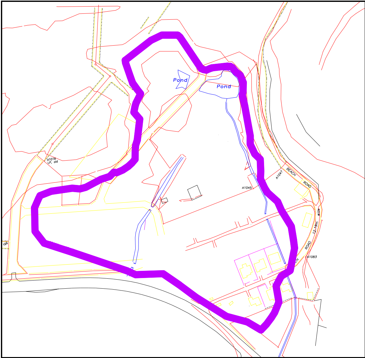
Figure 5: Demarcation of 100 year flood elevation of 17.48m
